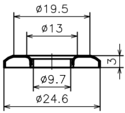
NYLON BUSH WEIGHT=1.30g
