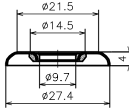
NYLON BUSH WEIGHT=2.80g
