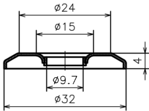
NYLON BUSH WEIGHT=4.50g
